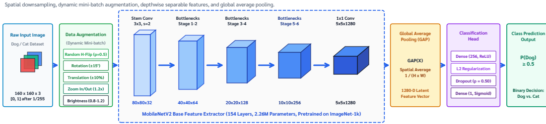
Figure 2(a): End-to-End Transfer Learning Computational & Tensor Pipeline
